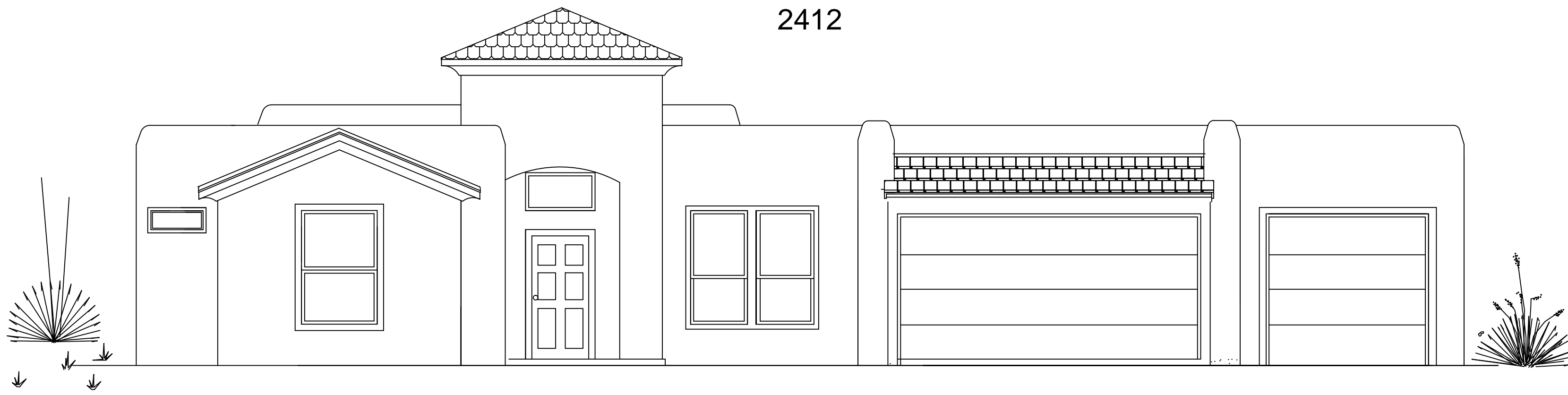
FRONT ELEVATION
