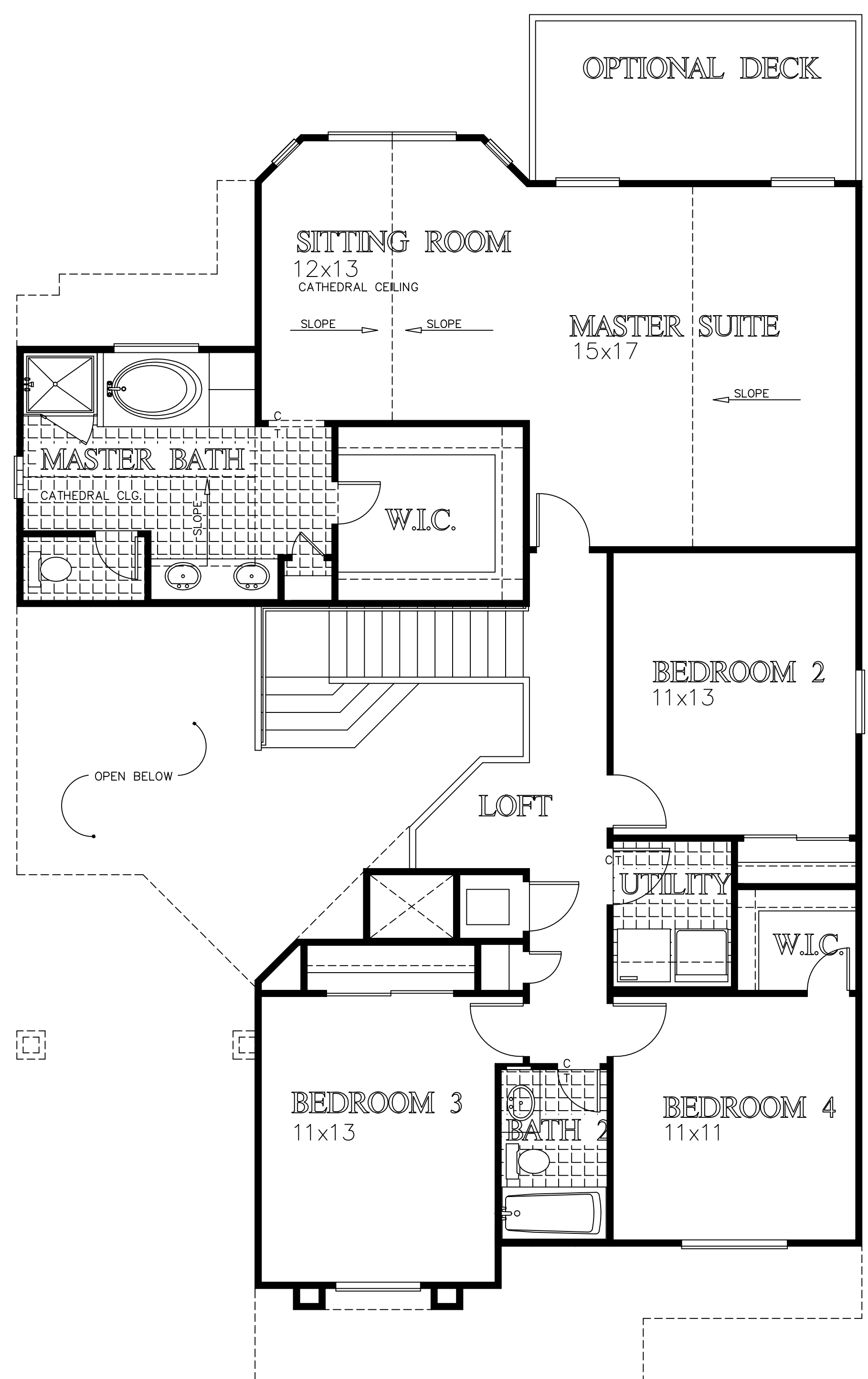
SECOND LEVEL FLOOR PLAN
