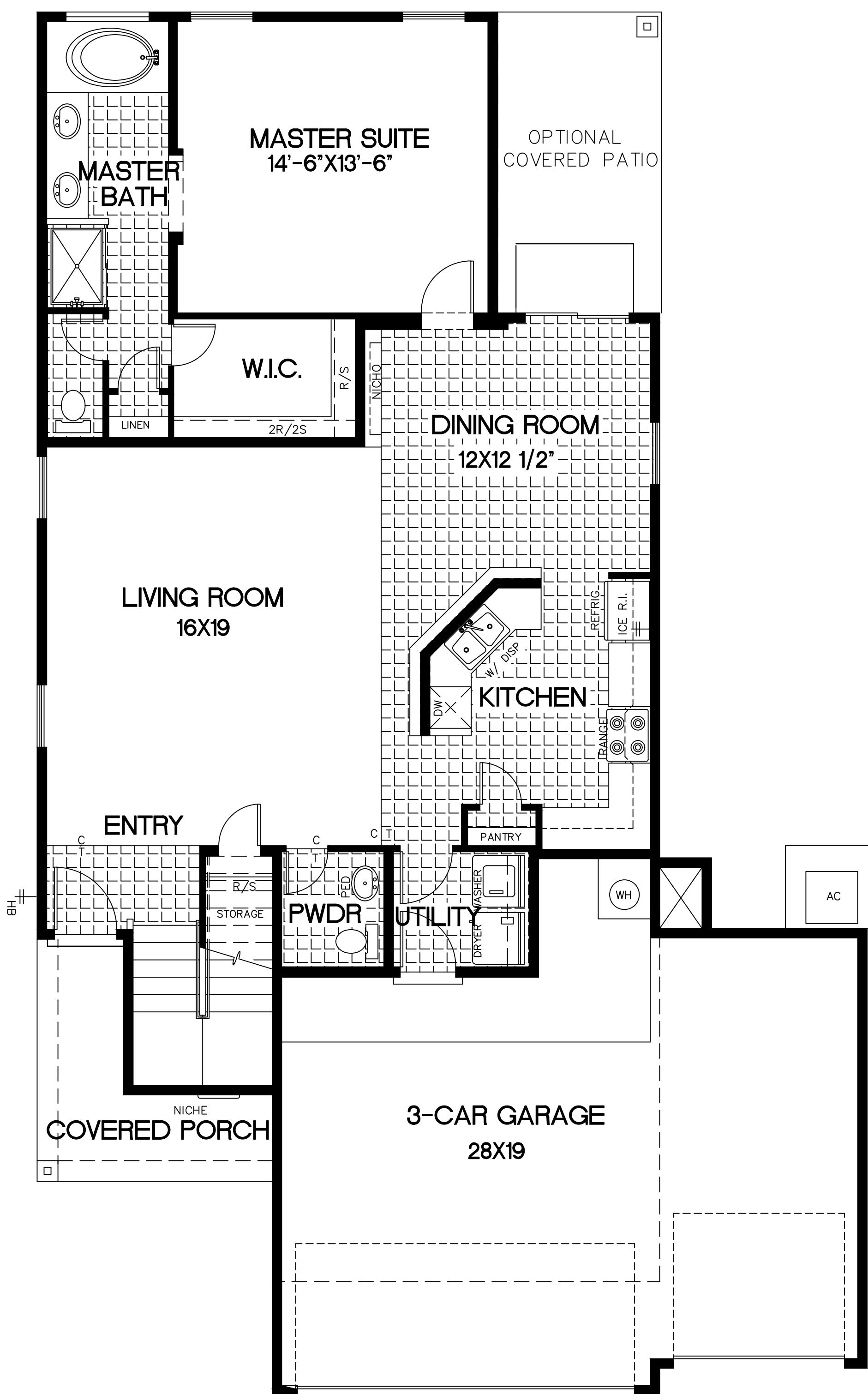
LOWER LEVEL A & B
