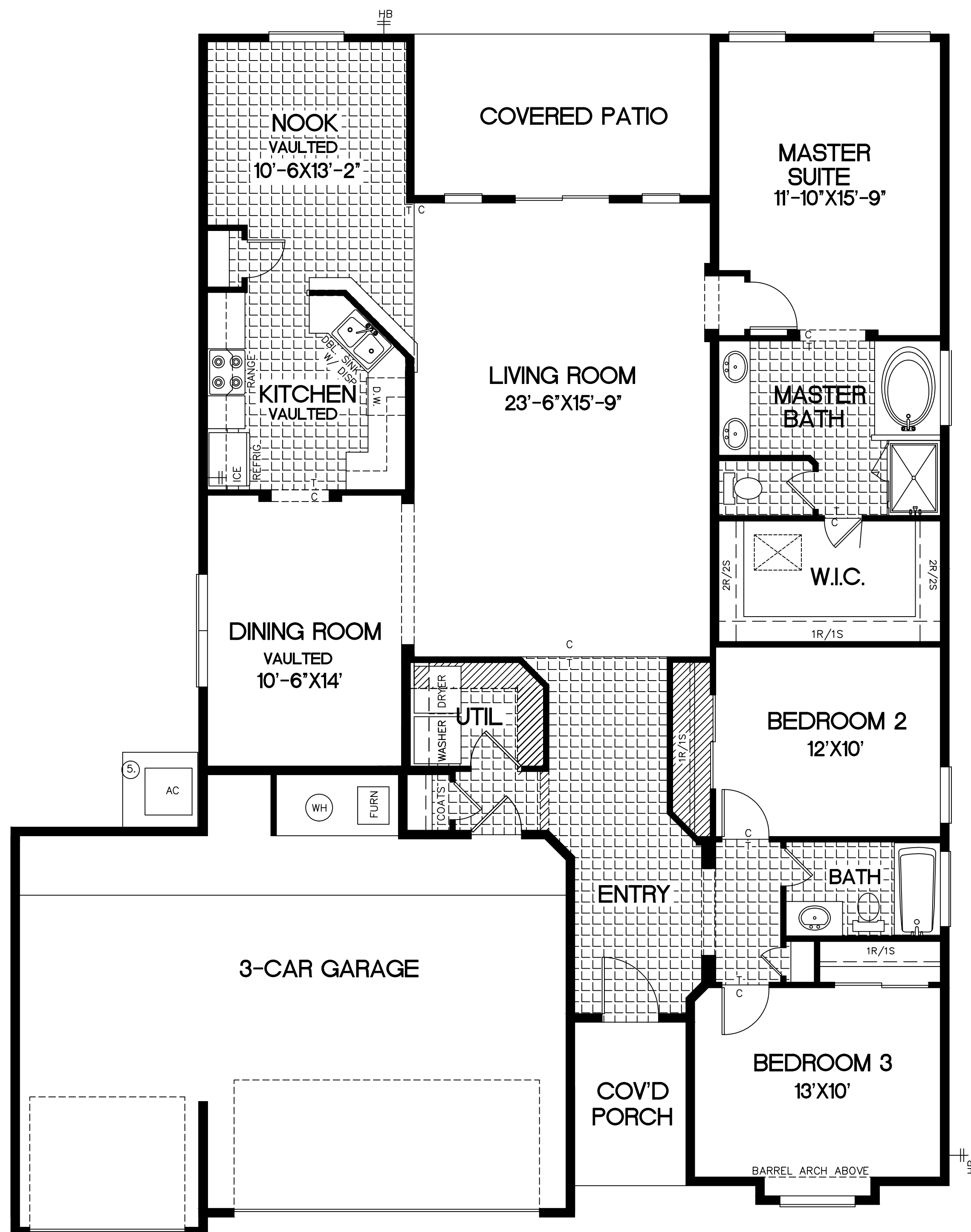
FLOOR PLAN A & B
